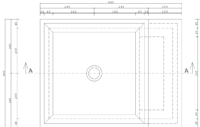
Floor plan
